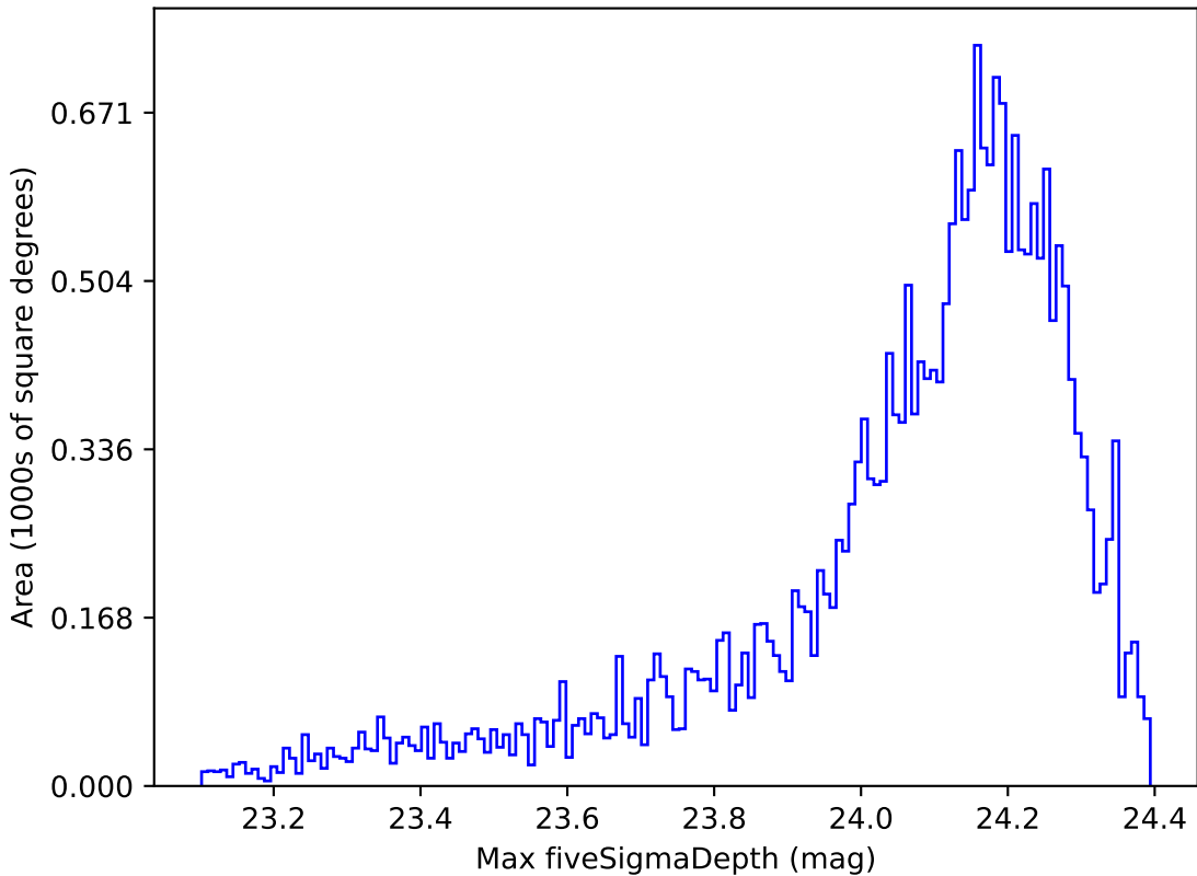
roll_pause_mjdp60_v3.4_10yrs Yr 1 i band: Max fiveSigmaDepth
