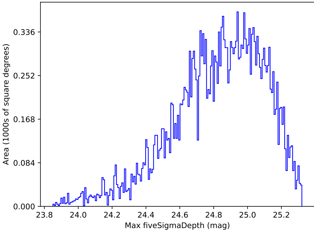
roll_pause_mjdp60_v3.4_10yrs Yr 1 all bands: Max fiveSigmaDepth
