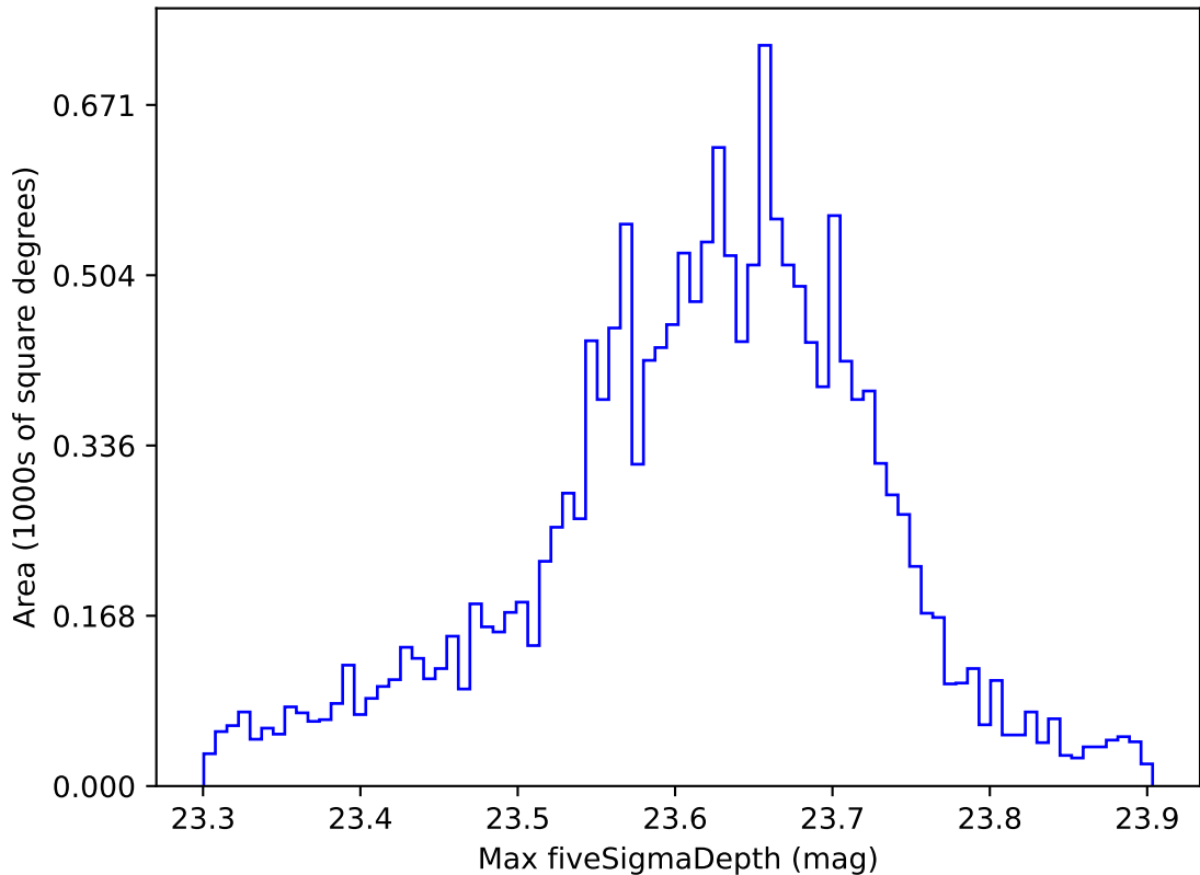
roll_pause_mjdp60_v3.4_10yrs WFD z band: Max fiveSigmaDepth
