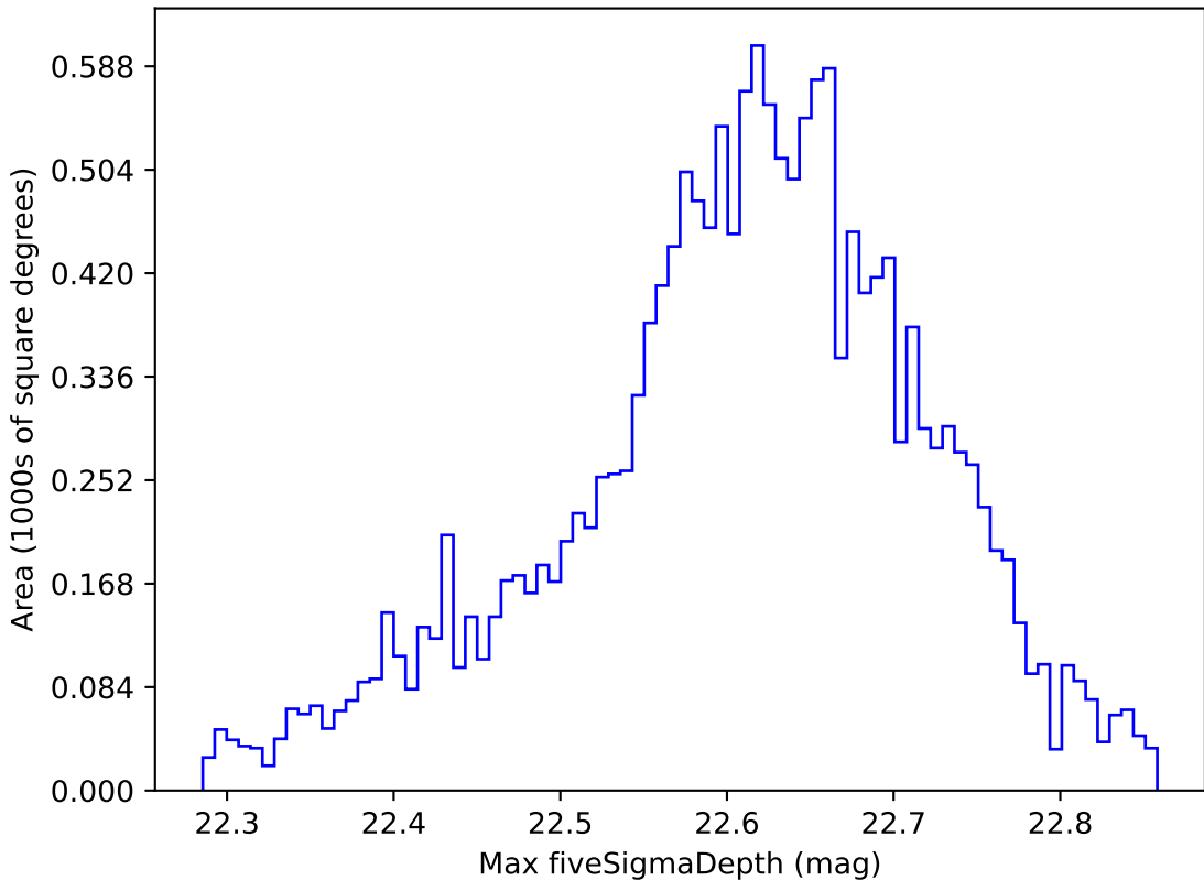
roll_pause_mjdp60_v3.4_10yrs WFD y band: Max fiveSigmaDepth
