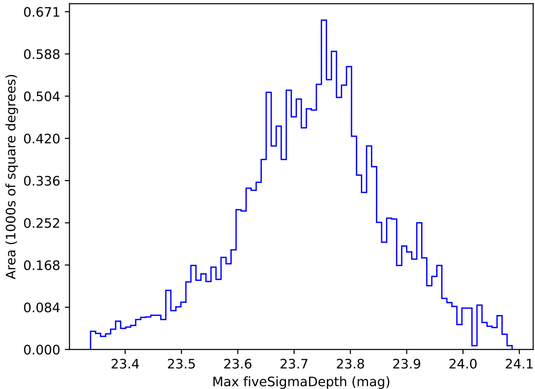
roll_pause_mjdp60_v3.4_10yrs WFD u band: Max fiveSigmaDepth
