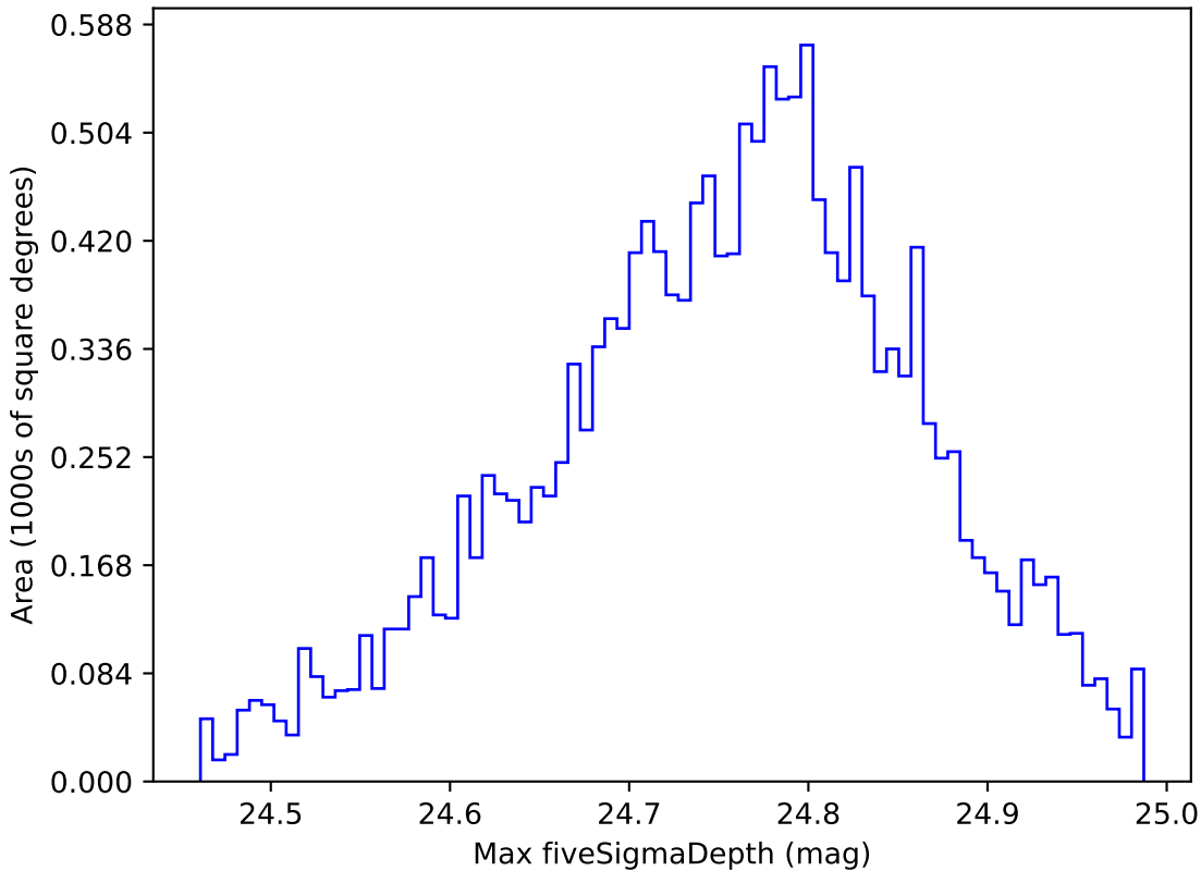
roll_pause_mjdp60_v3.4_10yrs WFD r band: Max fiveSigmaDepth
