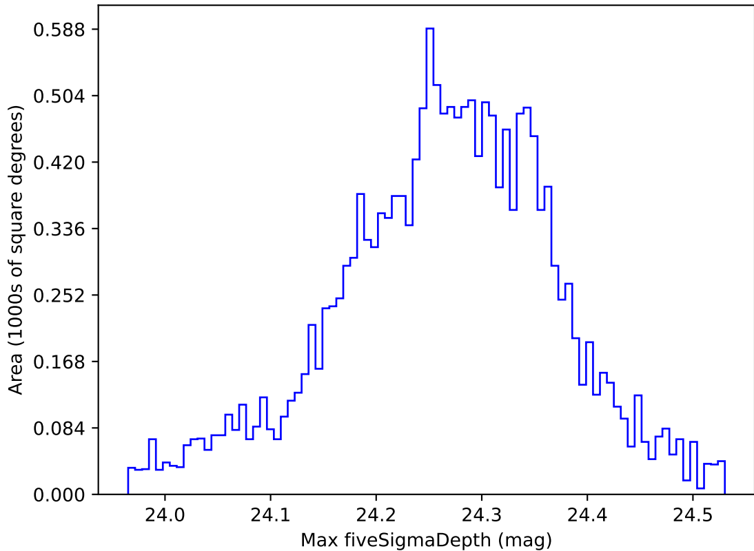
roll_pause_mjdp60_v3.4_10yrs WFD i band: Max fiveSigmaDepth
