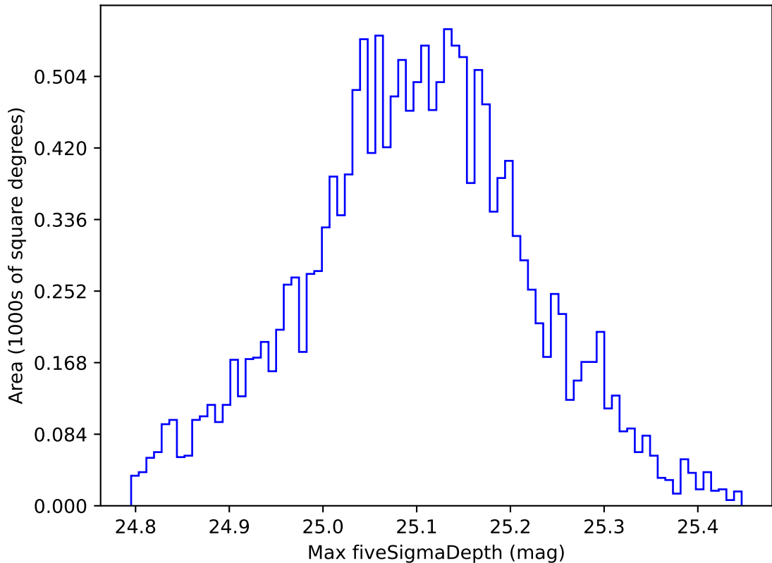
roll_pause_mjdp60_v3.4_10yrs WFD g band: Max fiveSigmaDepth
