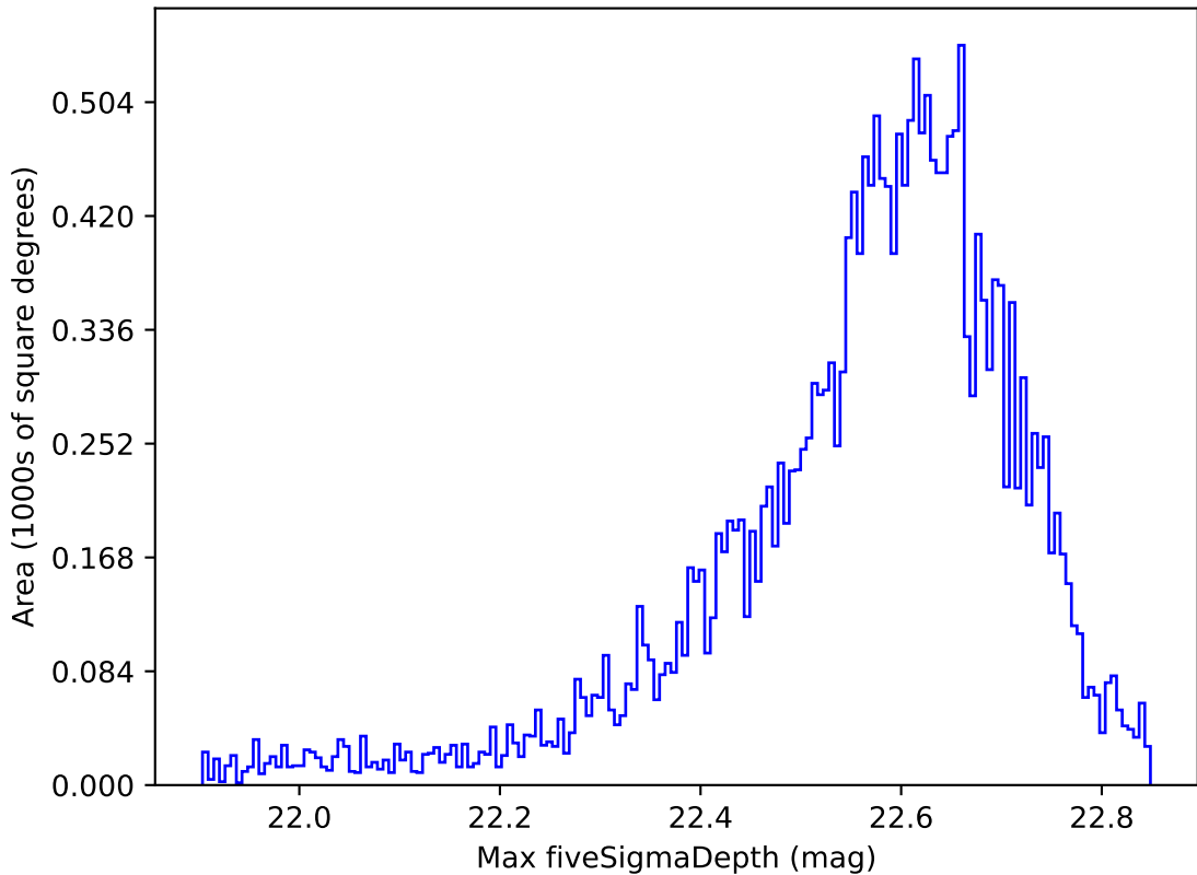
roll_pause_mjdp60_v3.4_10yrs All sky y band: Max fiveSigmaDepth
