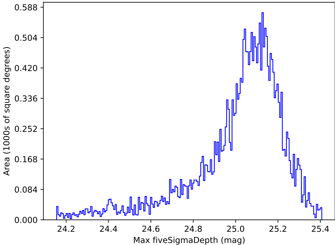
roll_pause_mjdp60_v3.4_10yrs All sky g band: Max fiveSigmaDepth
