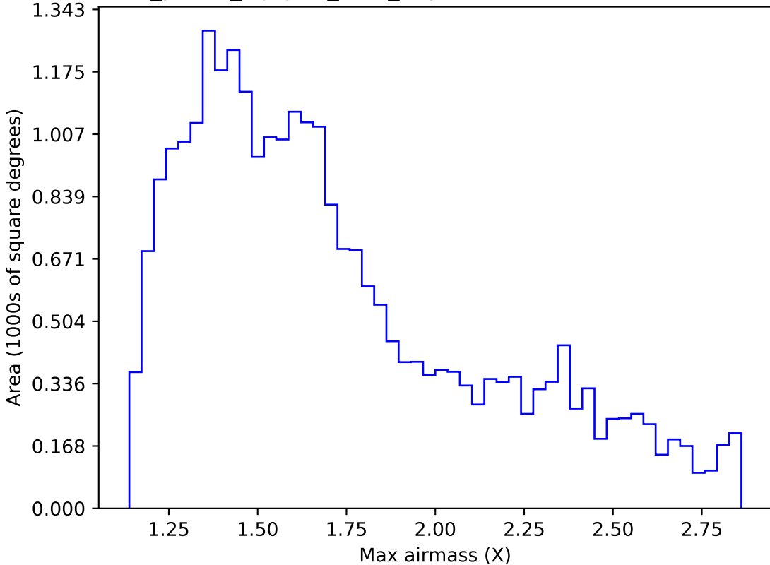
roll_pause_mjdp60_v3.4_10yrs Yr 1 z band: Max airmass
