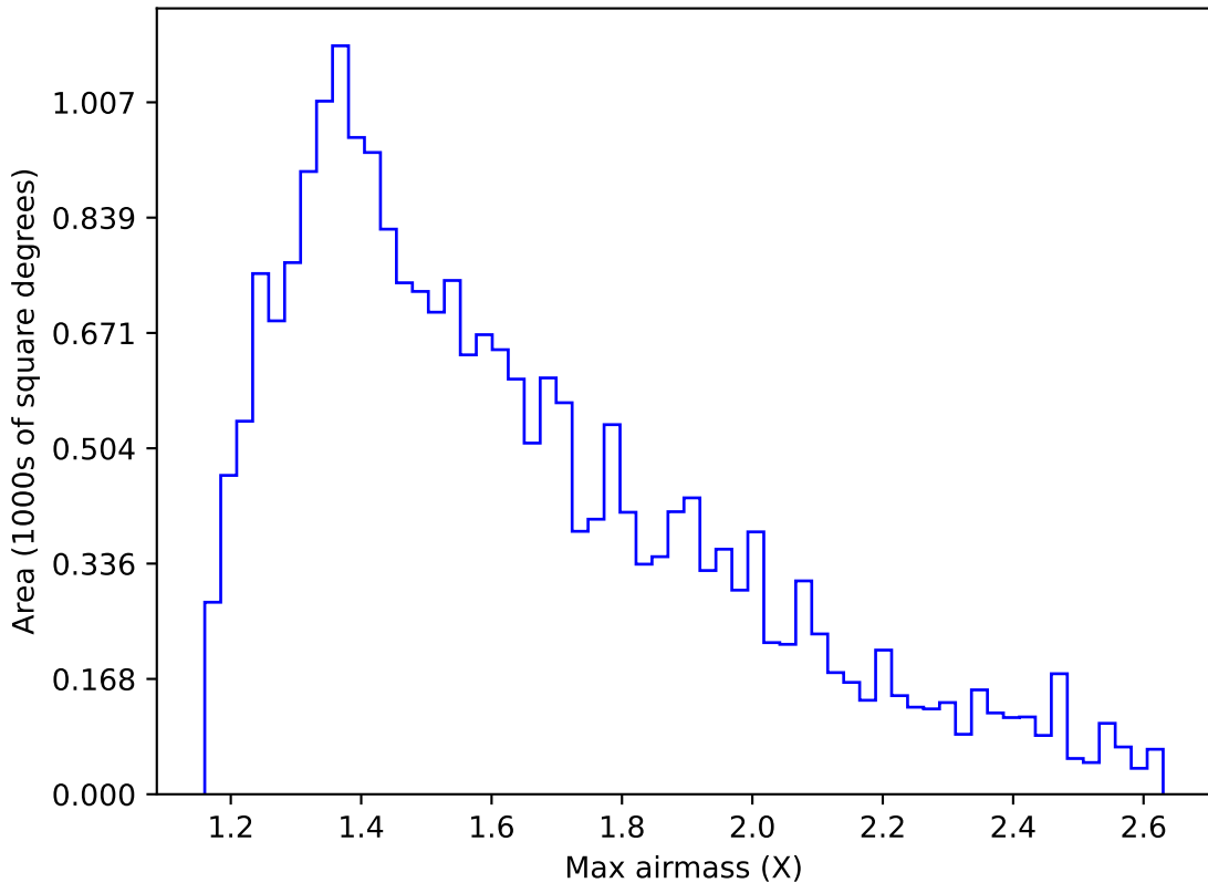
roll_pause_mjdp60_v3.4_10yrs Yr 1 y band: Max airmass
