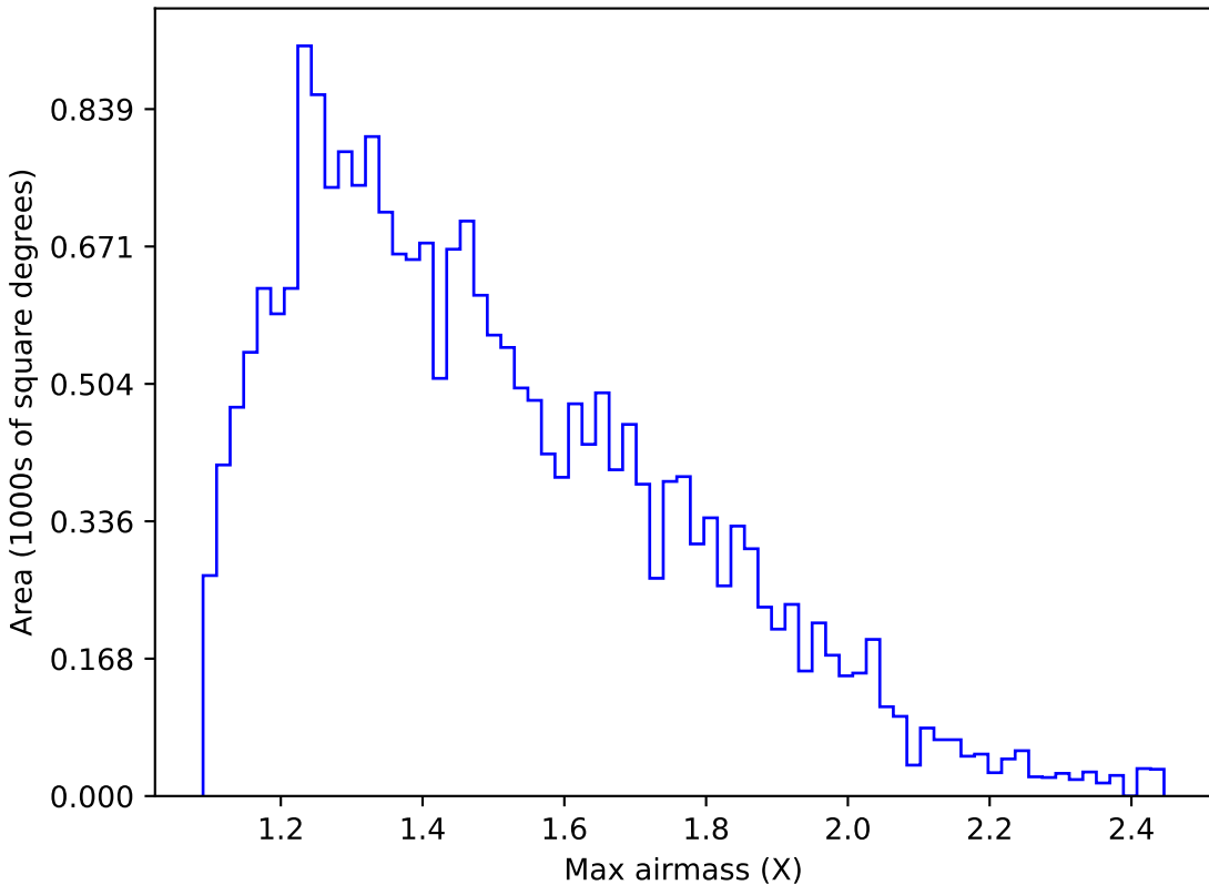
roll_pause_mjdp60_v3.4_10yrs Yr 1 u band: Max airmass
