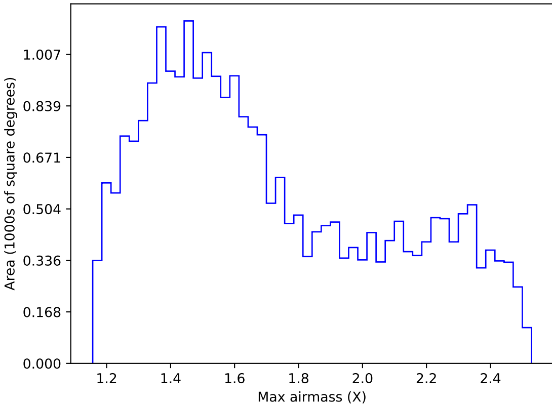
roll_pause_mjdp60_v3.4_10yrs Yr 1 r band: Max airmass
