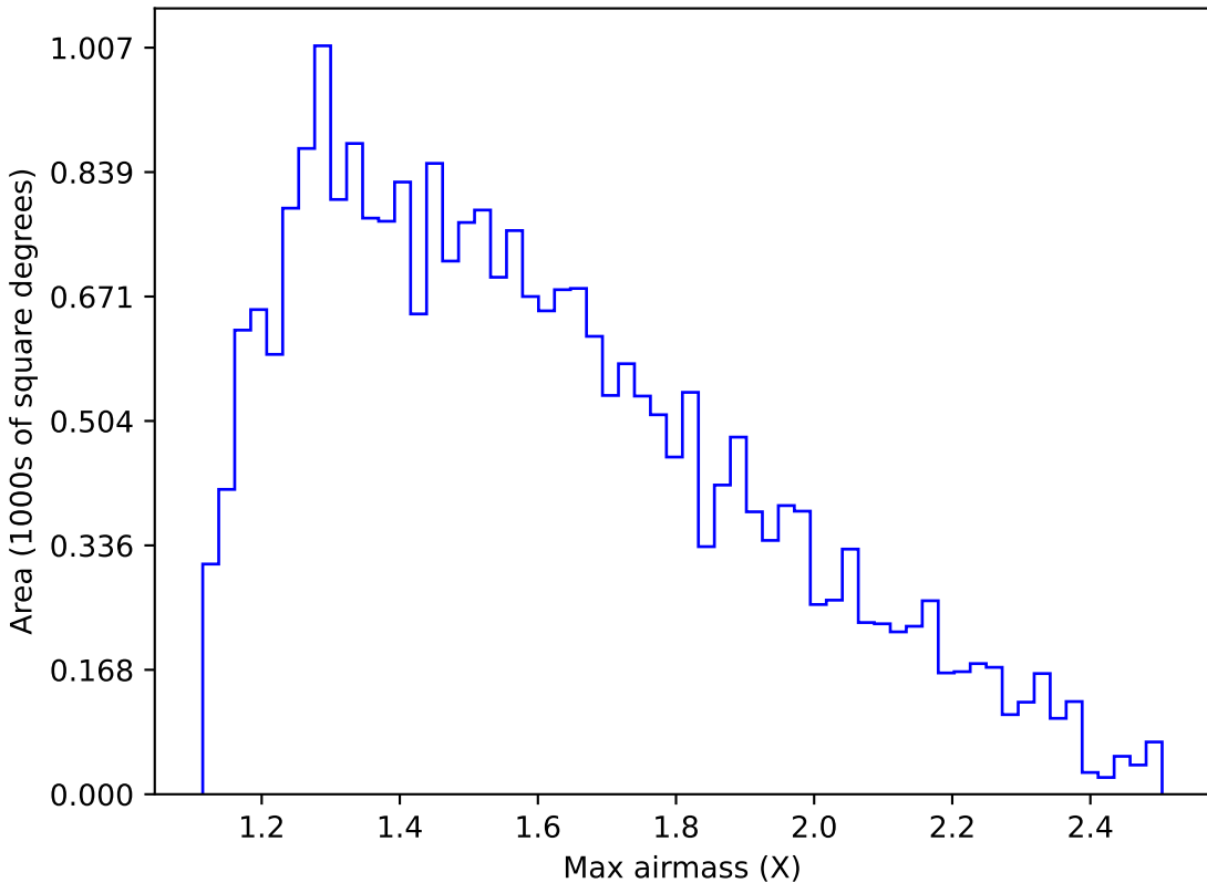
roll_pause_mjdp60_v3.4_10yrs Yr 1 g band: Max airmass
