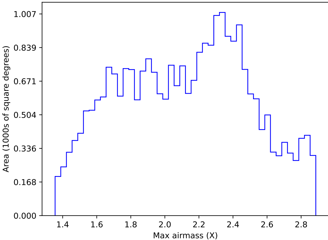
roll_pause_mjdp60_v3.4_10yrs Yr 1 all bands: Max airmass
