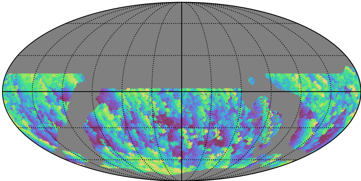
roll_pause_mjdp60_v3.4_10yrs WFD y band: Max airmass
