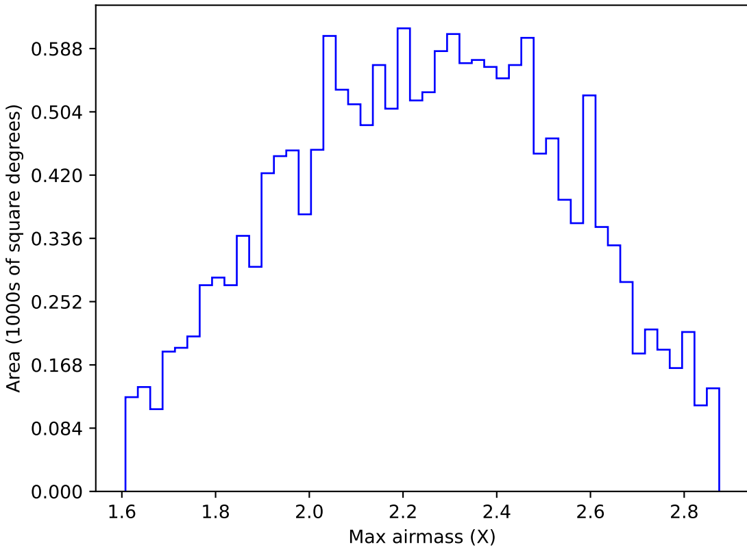
roll_pause_mjdp60_v3.4_10yrs WFD y band: Max airmass
