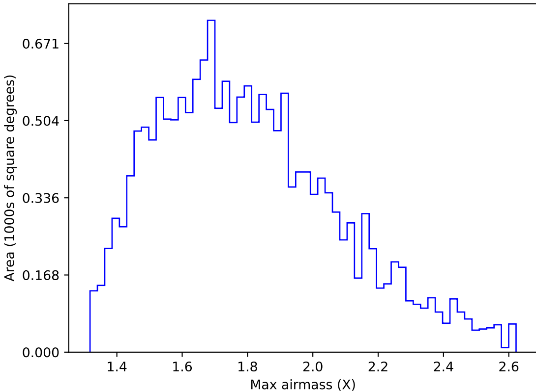
roll_pause_mjdp60_v3.4_10yrs WFD u band: Max airmass
