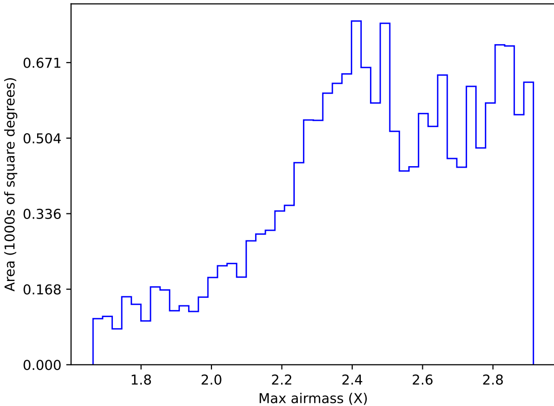
roll_pause_mjdp60_v3.4_10yrs WFD i band: Max airmass
