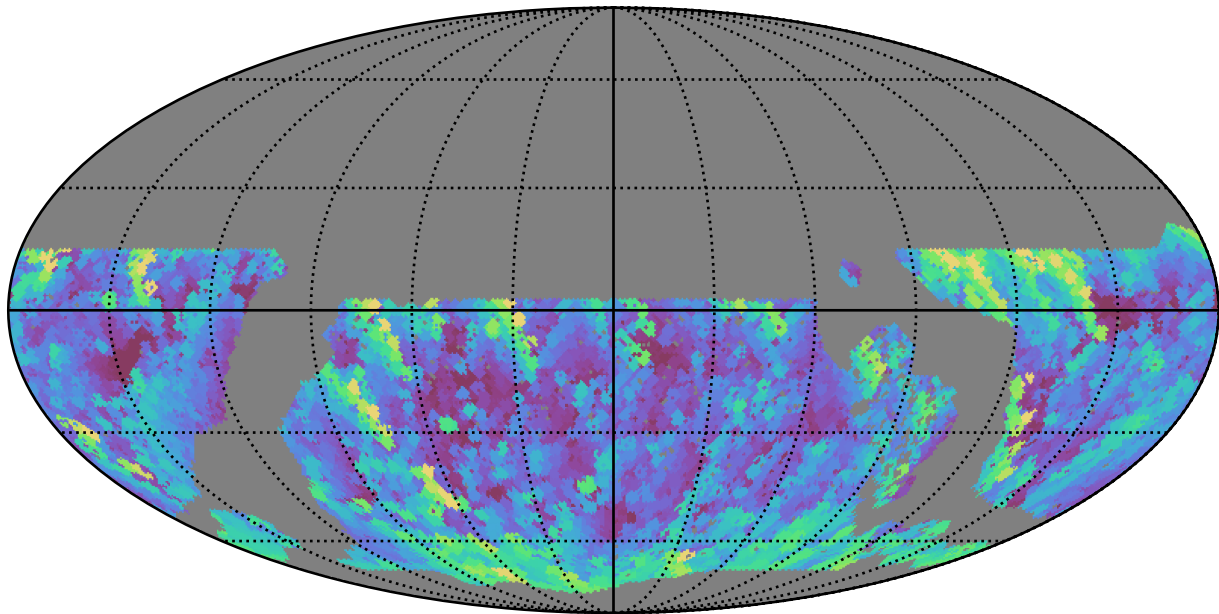
roll_pause_mjdp60_v3.4_10yrs WFD g band: Max airmass
