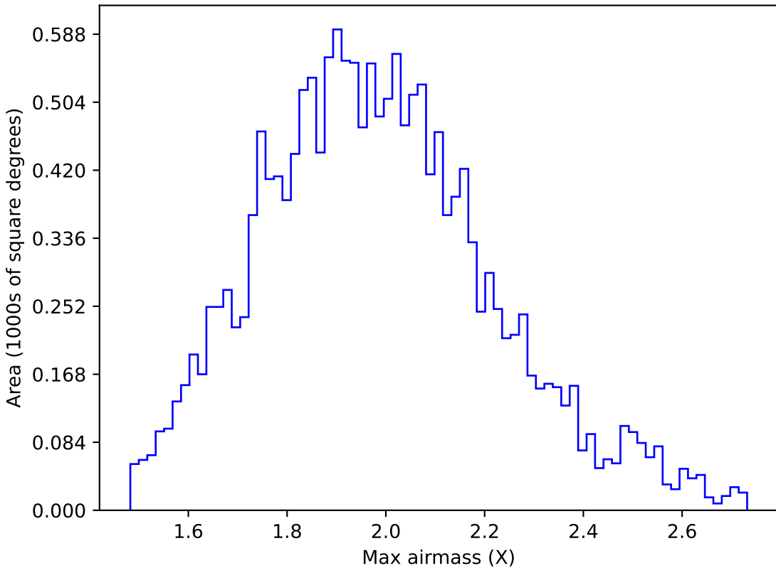
roll_pause_mjdp60_v3.4_10yrs WFD g band: Max airmass
