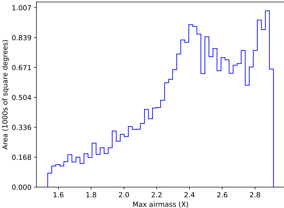
roll_pause_mjdp60_v3.4_10yrs All sky z band: Max airmass
