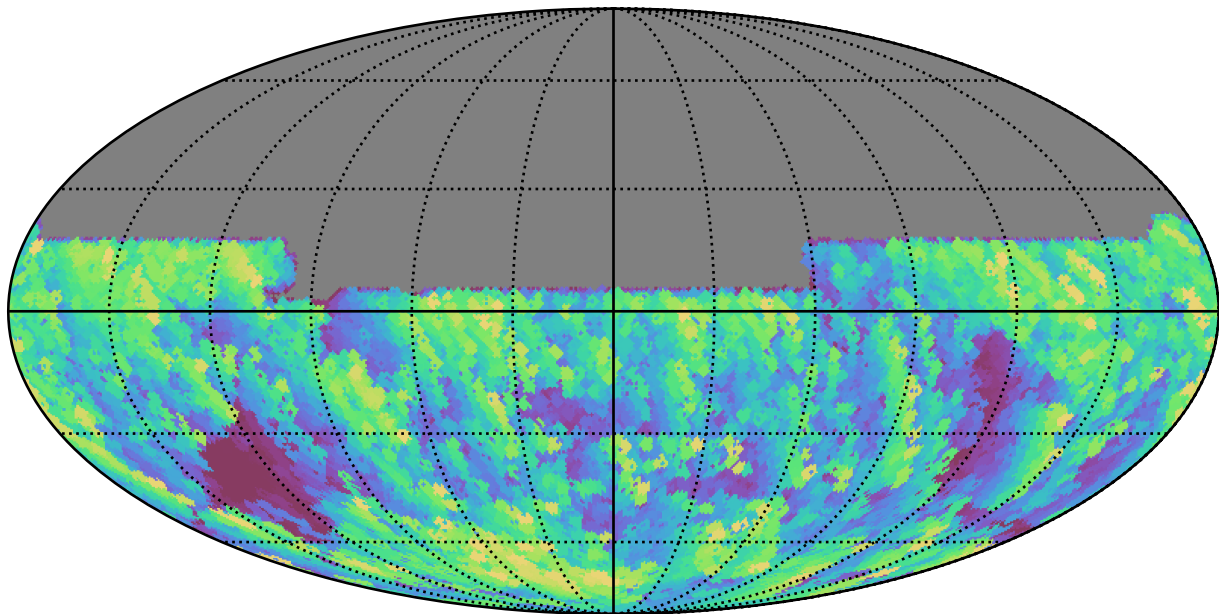
roll_pause_mjdp60_v3.4_10yrs All sky y band: Max airmass
