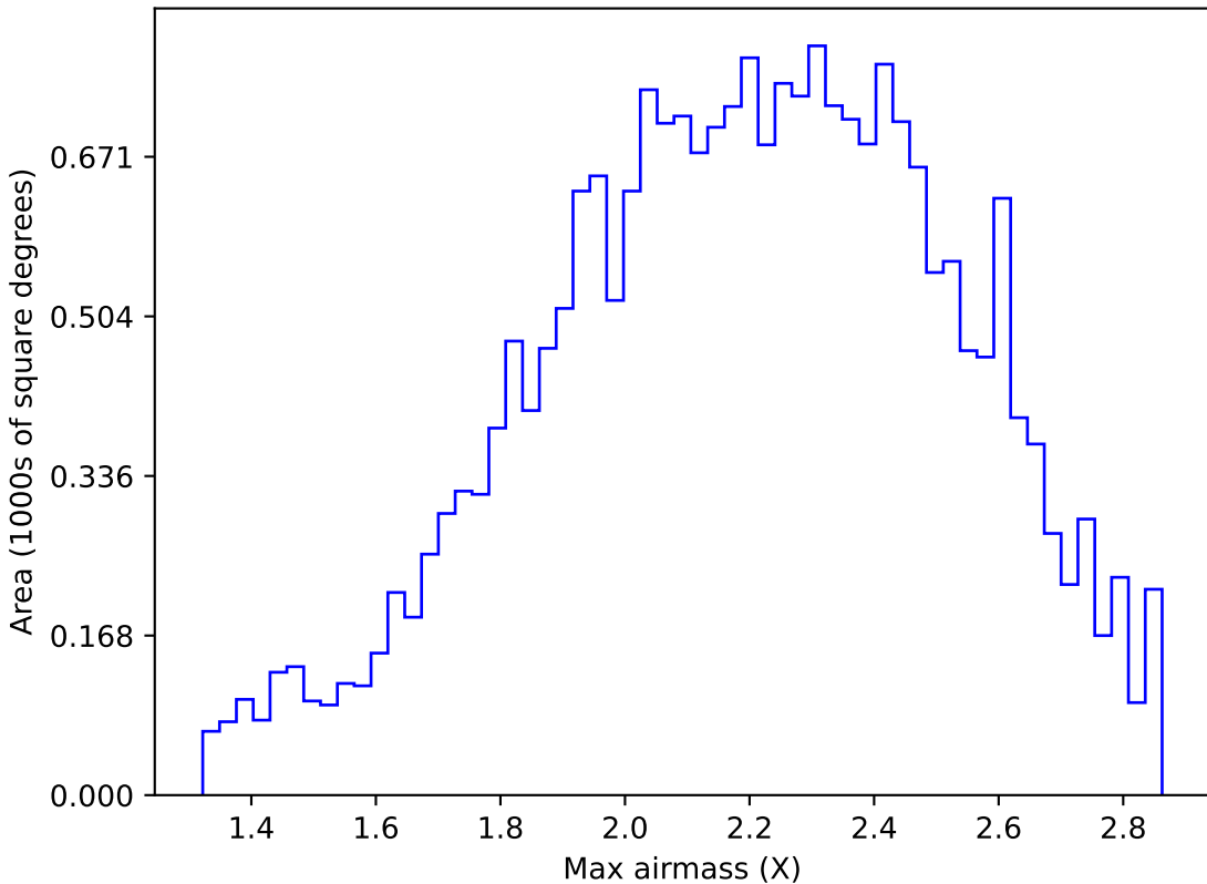
roll_pause_mjdp60_v3.4_10yrs All sky y band: Max airmass
