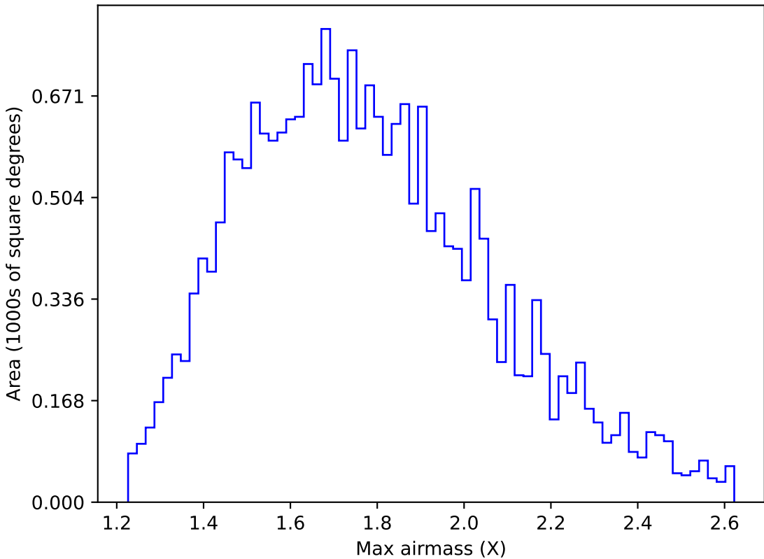
roll_pause_mjdp60_v3.4_10yrs All sky u band: Max airmass
