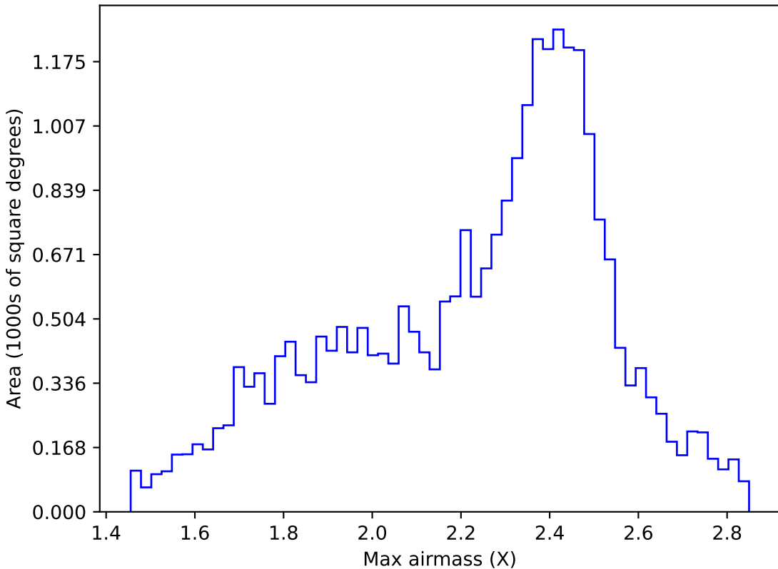
roll_pause_mjdp60_v3.4_10yrs All sky r band: Max airmass
