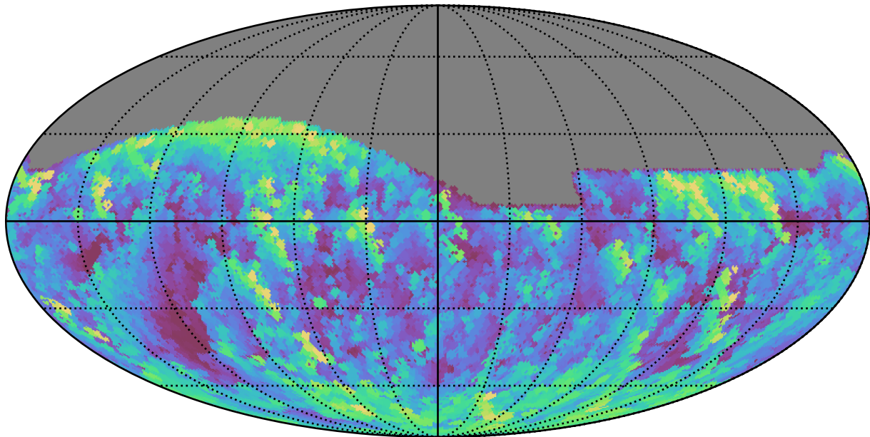
roll_pause_mjdp60_v3.4_10yrs All sky g band: Max airmass
