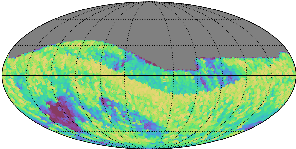
roll_pause_mjdp60_v3.4_10yrs All sky all bands: Max airmass
