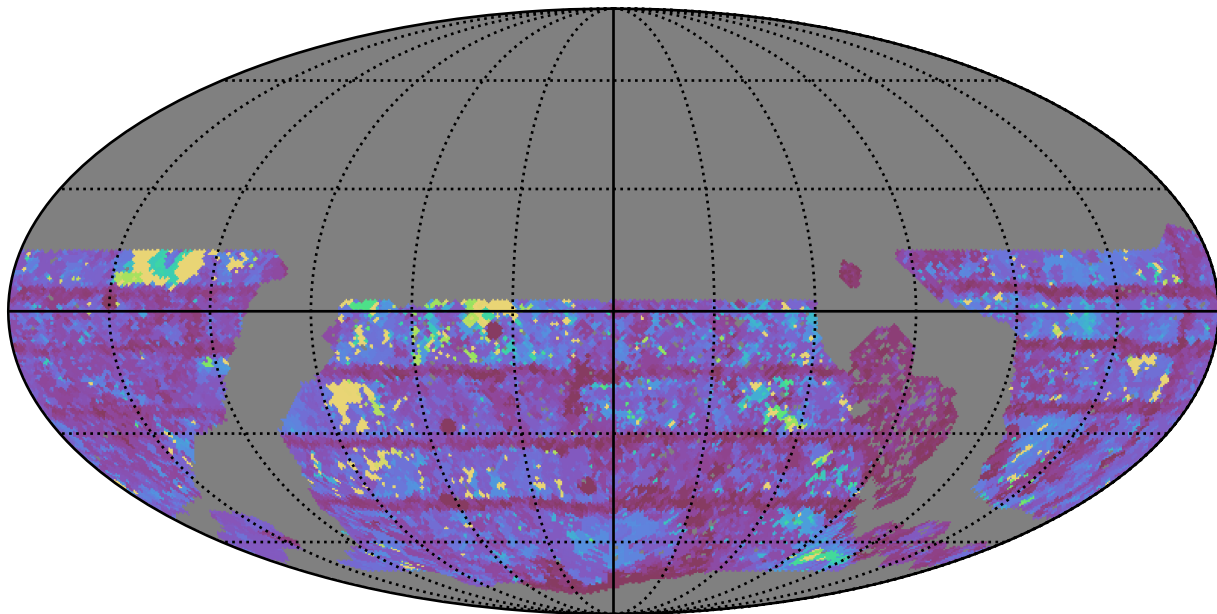
roll_pause_mjdp60_v3.4_10yrs WFD z band: Max Inter-Night Gap
