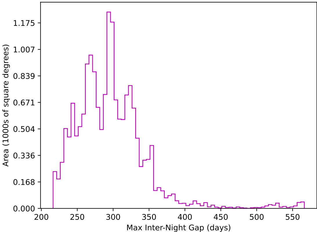
roll_pause_mjdp60_v3.4_10yrs WFD z band: Max Inter-Night Gap
