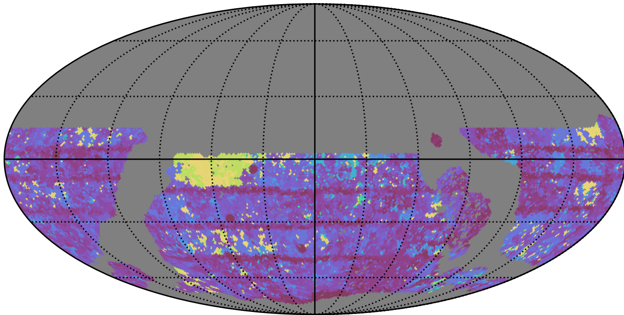
roll_pause_mjdp60_v3.4_10yrs WFD y band: Max Inter-Night Gap
