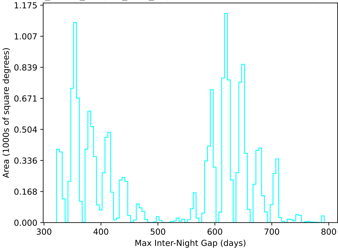
roll_pause_mjdp60_v3.4_10yrs WFD u band: Max Inter-Night Gap
