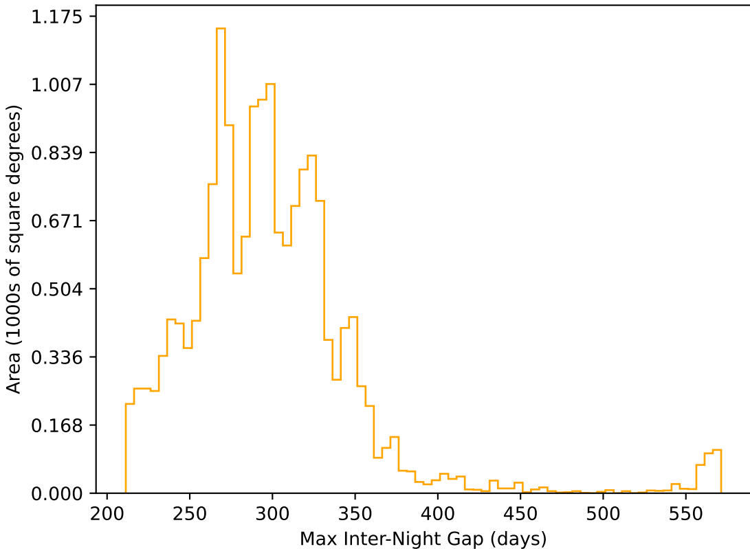
roll_pause_mjdp60_v3.4_10yrs WFD r band: Max Inter-Night Gap
