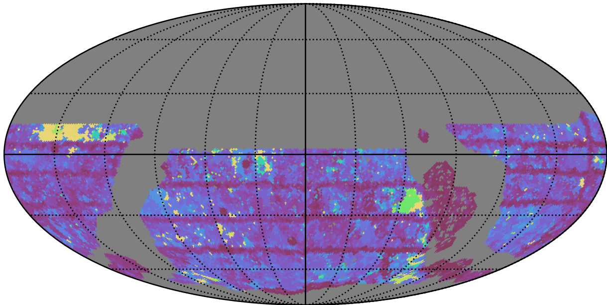
roll_pause_mjdp60_v3.4_10yrs WFD i band: Max Inter-Night Gap
