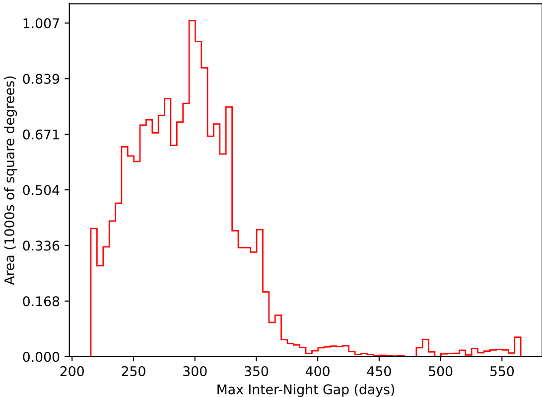
roll_pause_mjdp60_v3.4_10yrs WFD i band: Max Inter-Night Gap
