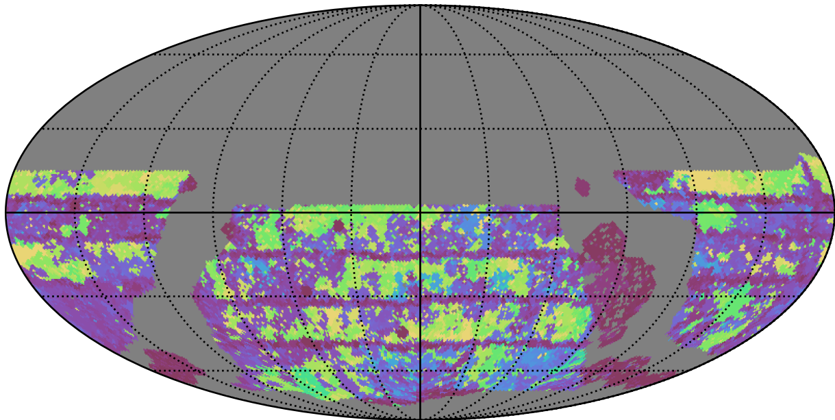
roll_pause_mjdp60_v3.4_10yrs WFD g band: Max Inter-Night Gap
