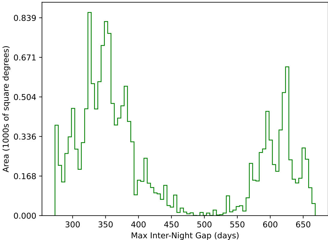
roll_pause_mjdp60_v3.4_10yrs WFD g band: Max Inter-Night Gap
