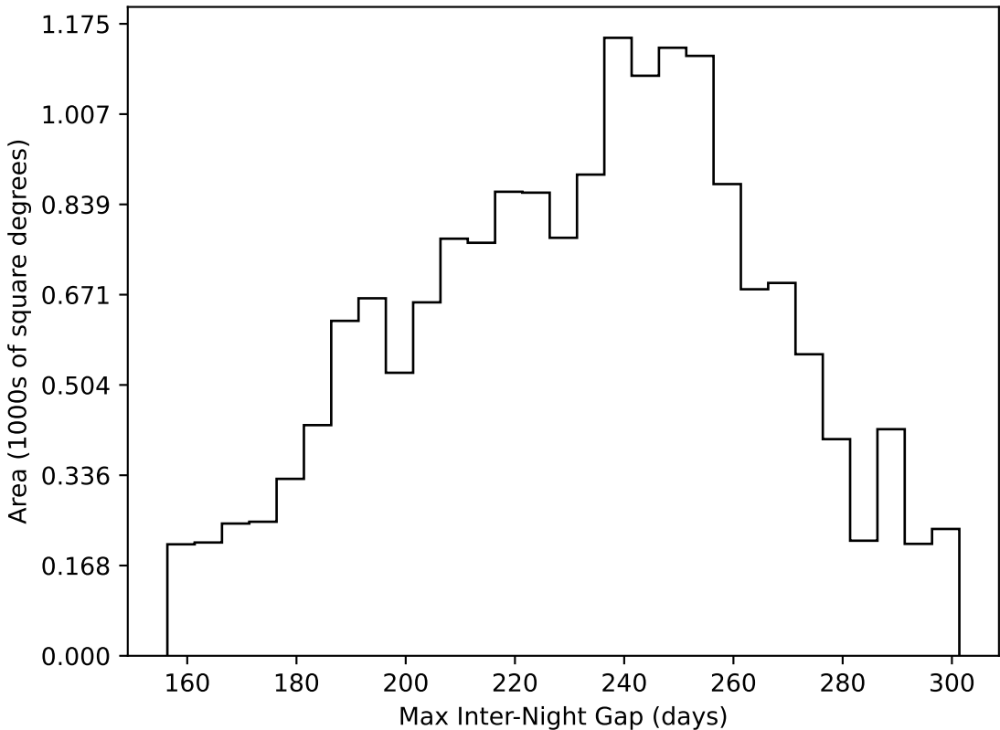
roll_pause_mjdp60_v3.4_10yrs WFD all bands: Max Inter-Night Gap
