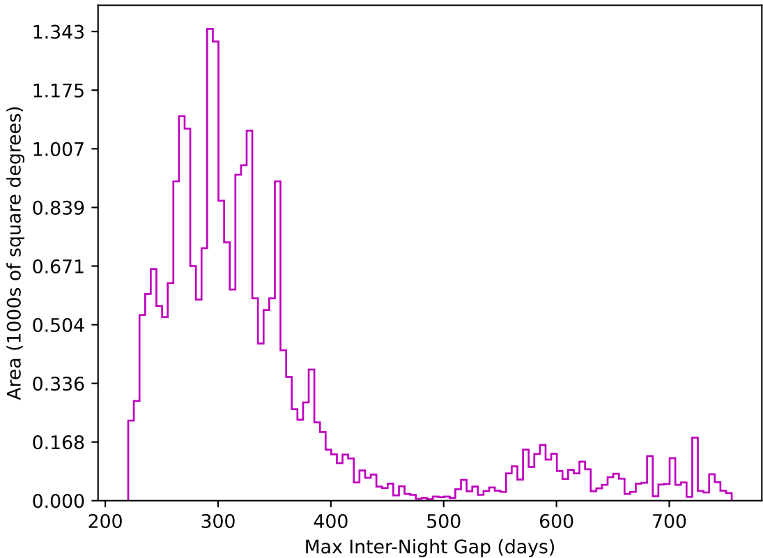
roll_pause_mjdp60_v3.4_10yrs All sky z band: Max Inter-Night Gap
