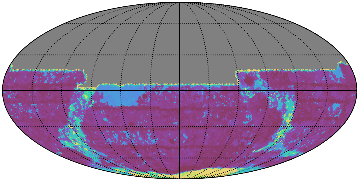
roll_pause_mjdp60_v3.4_10yrs All sky y band: Max Inter-Night Gap
