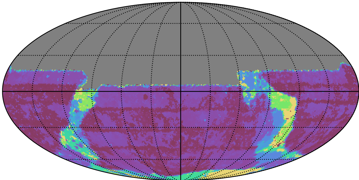
roll_pause_mjdp60_v3.4_10yrs All sky u band: Max Inter-Night Gap
