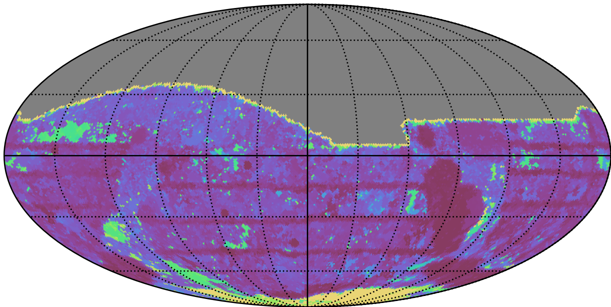
roll_pause_mjdp60_v3.4_10yrs All sky r band: Max Inter-Night Gap
