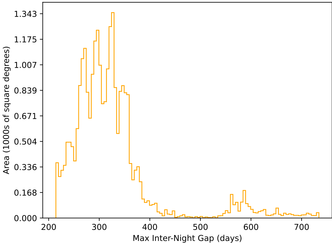
roll_pause_mjdp60_v3.4_10yrs All sky r band: Max Inter-Night Gap
