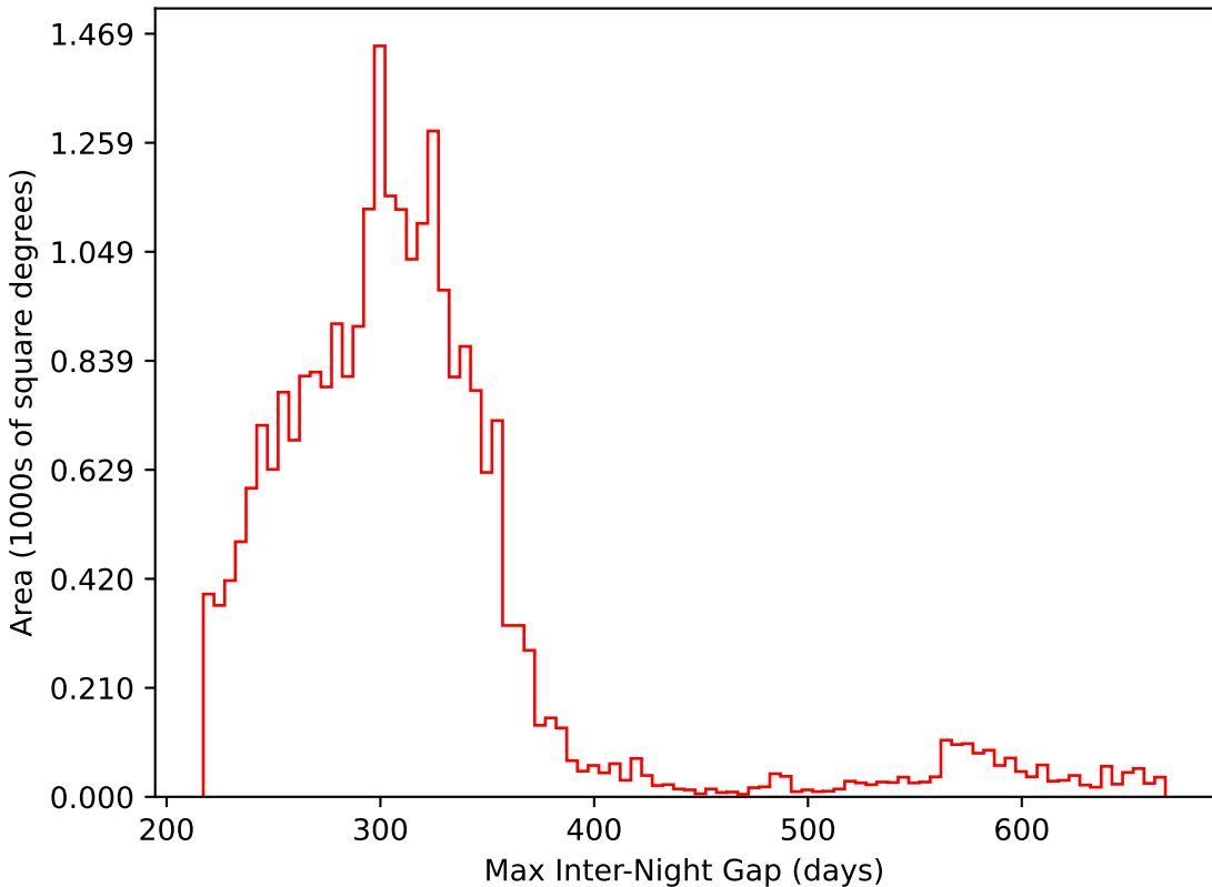
roll_pause_mjdp60_v3.4_10yrs All sky i band: Max Inter-Night Gap
