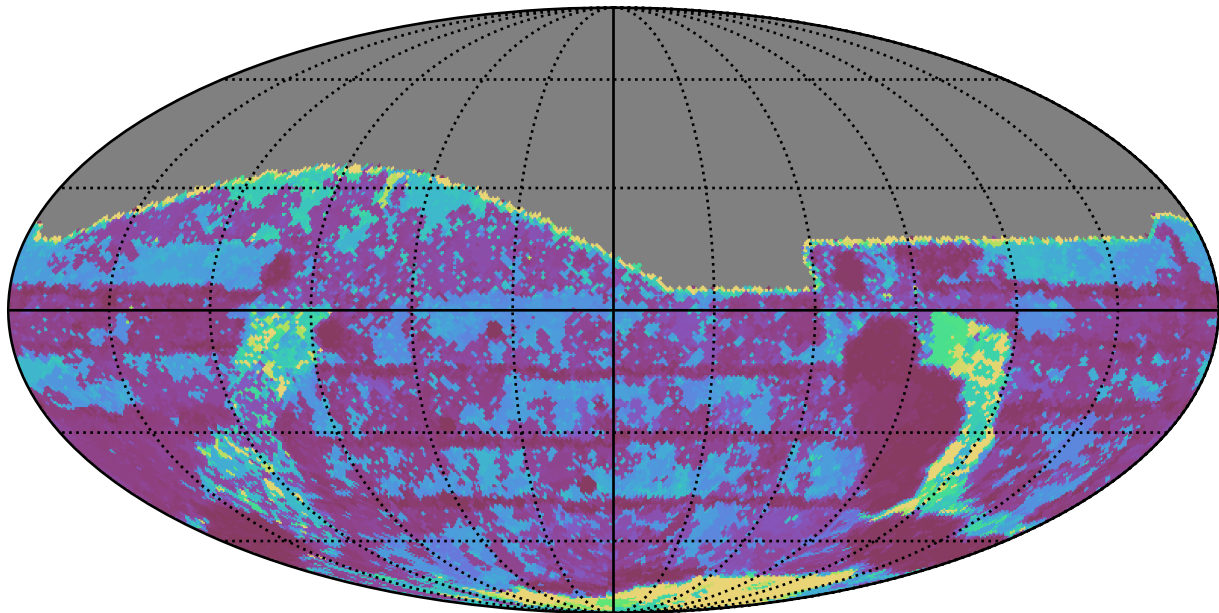
roll_pause_mjdp60_v3.4_10yrs All sky g band: Max Inter-Night Gap
