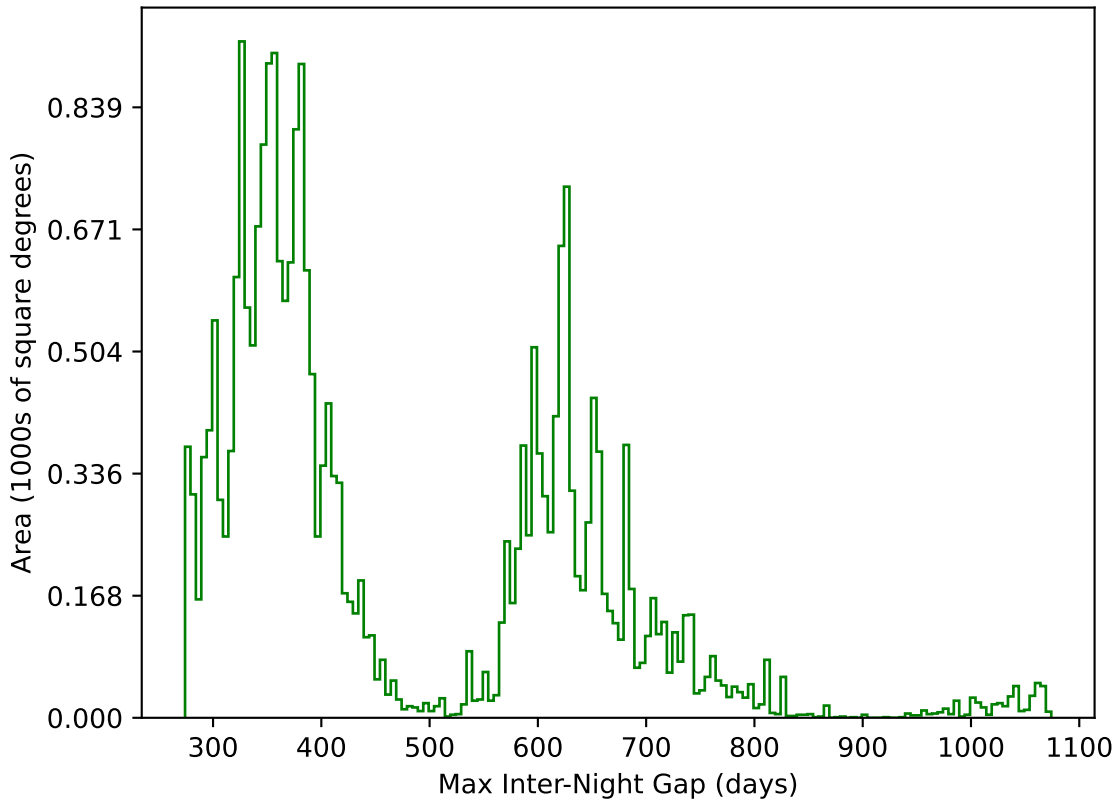
roll_pause_mjdp60_v3.4_10yrs All sky g band: Max Inter-Night Gap
