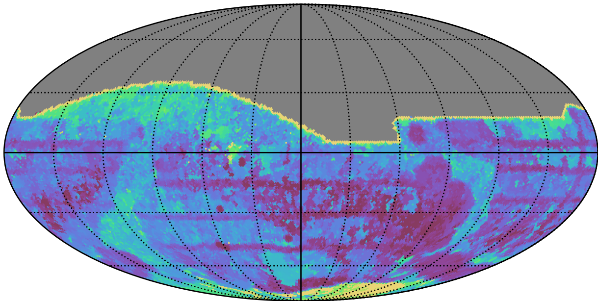
roll_pause_mjdp60_v3.4_10yrs All sky all bands: Max Inter-Night Gap
