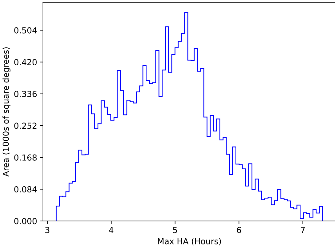
roll_pause_mjdp60_v3.4_10yrs WFD z band: Max HA
