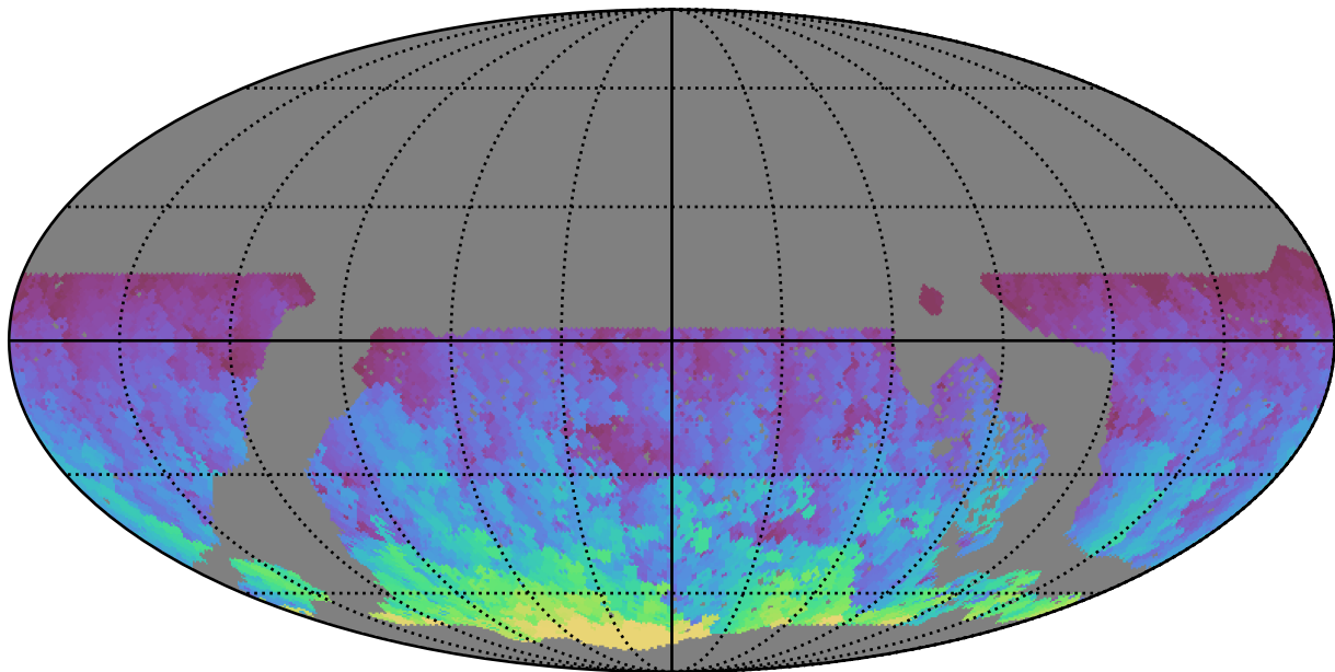
roll_pause_mjdp60_v3.4_10yrs WFD y band: Max HA
